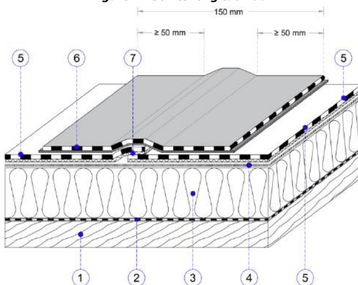
Figure 4 - Joints longitudinaux
